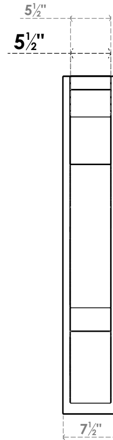
FRONT PROFILE
