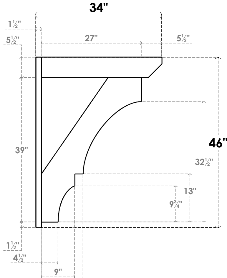
SIDE PROFILE
